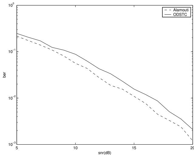
Fig. 2. Bit-error performance for ODSTC transmitting at a rate of 2.0 b/s/Hz. Also shown is the rate 2.0 Alamouti code with coherent detection.
