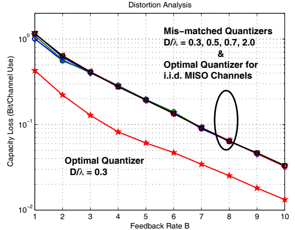
Fig. 2. Capacity loss of mismatched MISO quantizers with codebook designed for i.i.d. channels used in correlated fading channels
