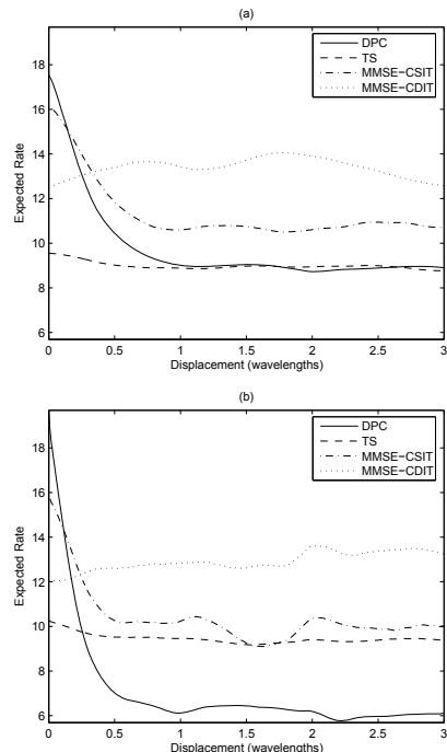
Fig. 4. Capacity degradation versus displacement for DPC, fair TS, MMSE-CSIT, and MMSE-CDIT for the ad hoc network in a) Open Field and b) Urban environments. Simulations were performed at 10 dB SNR with N_t = 4 transmit antenna, N_r = 4 receive antennas, and K = 6 users.
